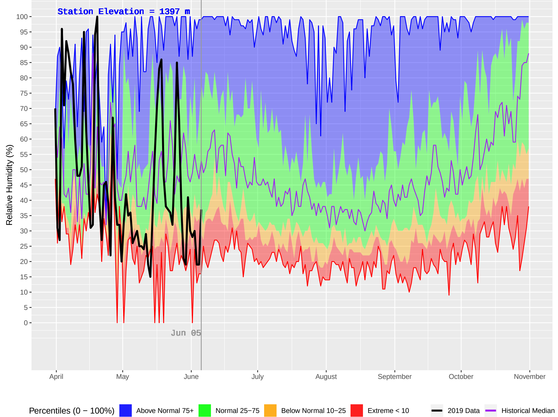
NANCY GREEN (407) : Historical (1992–2018) and Current (2019) Daily Relative Humidity
