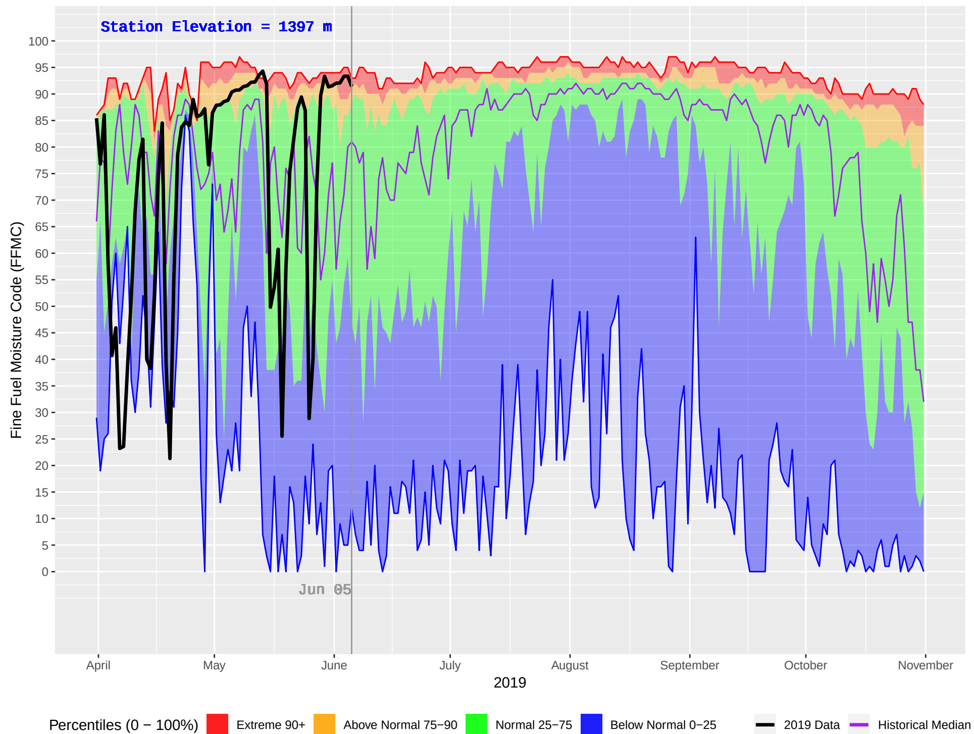
NANCY GREEN (407) : Historical (1992–2018) and Current (2019) Daily Fine Fuel Moisture Code (FFMC)
