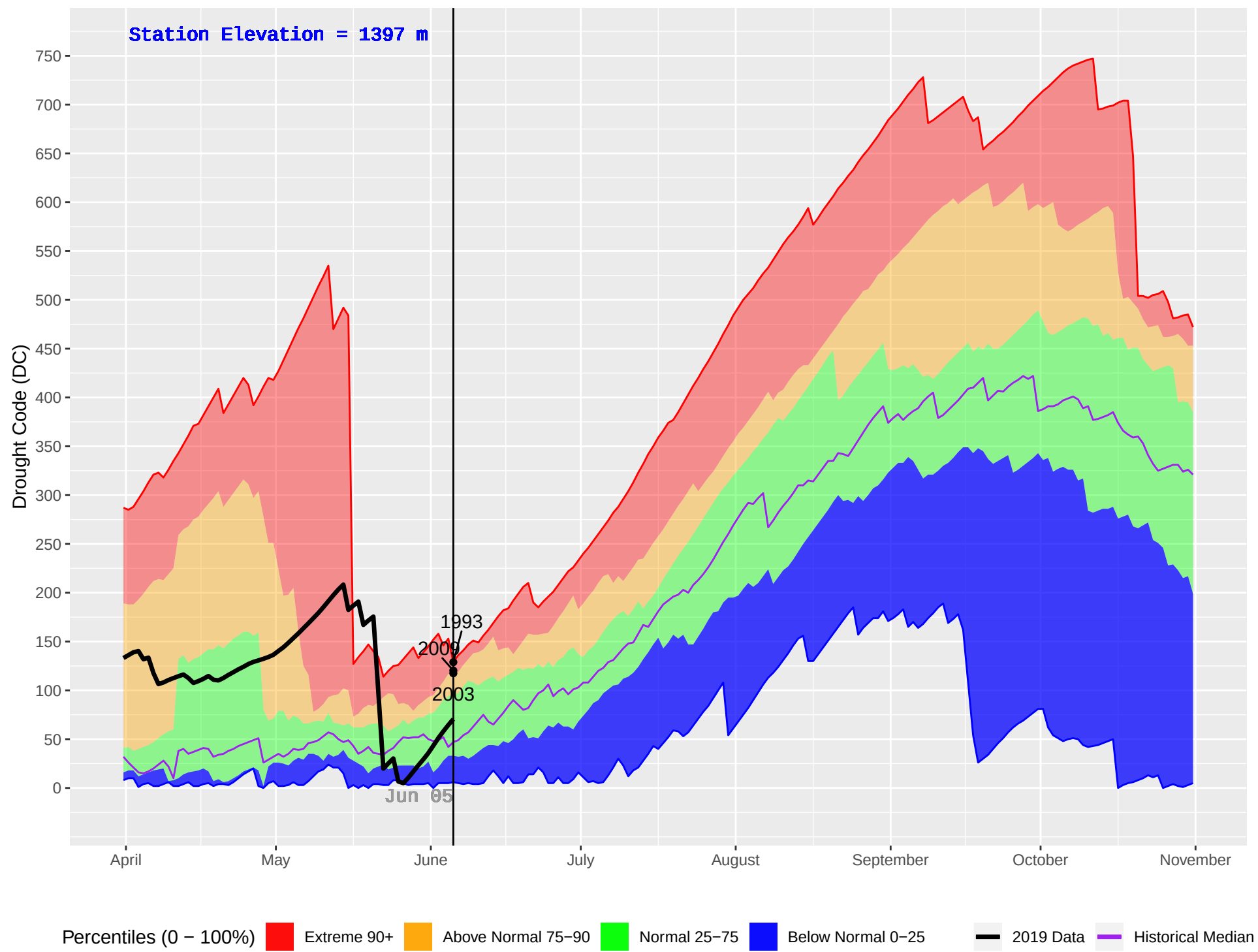
NANCY GREEN (407) : Historical (1992–2018) and Current (2019) Daily Drought Code (DC)
