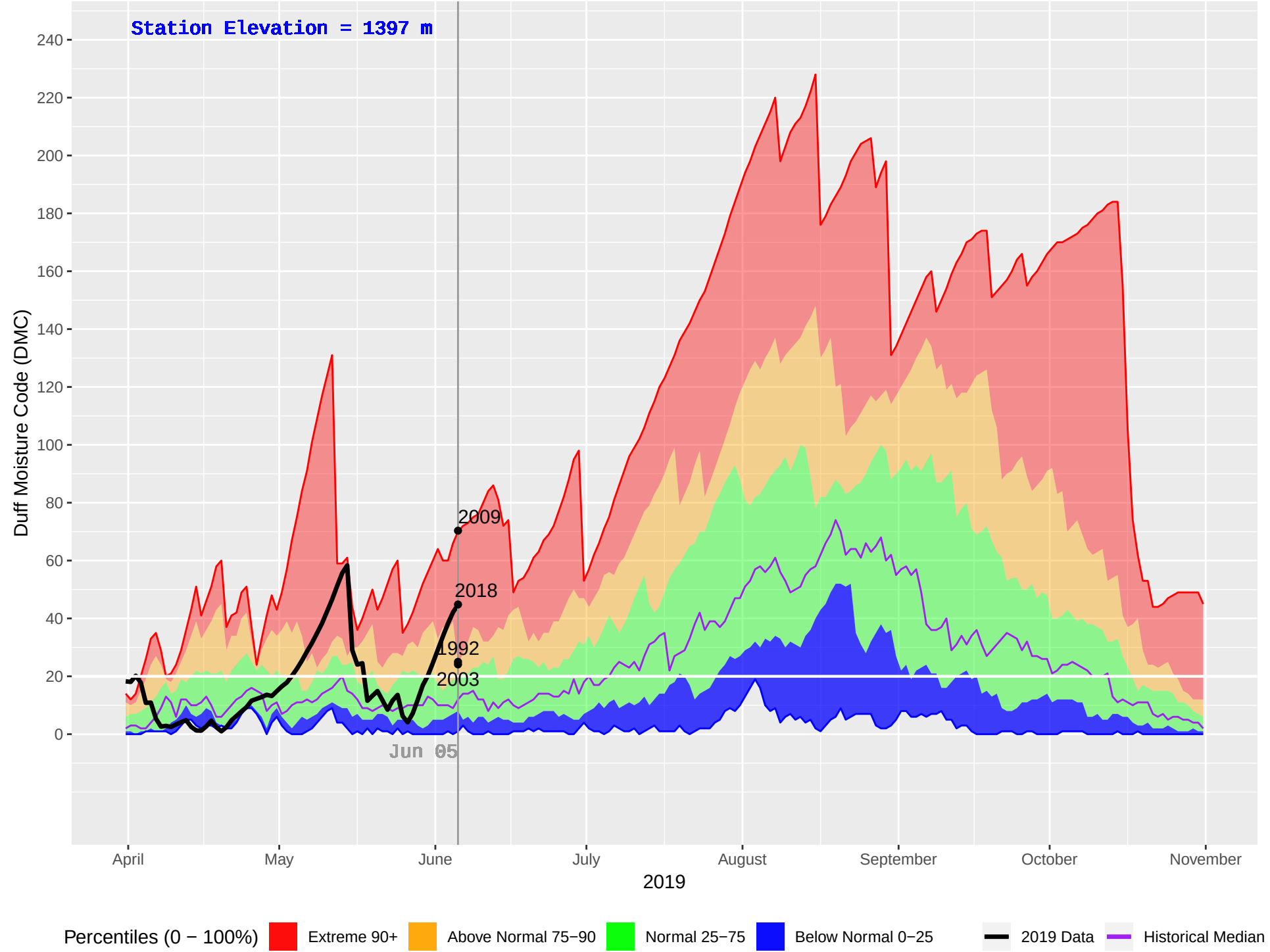
NANCY GREEN (407) : Historical (1992–2018), Current (2019) Daily Duff Moisture Code (DMC)
