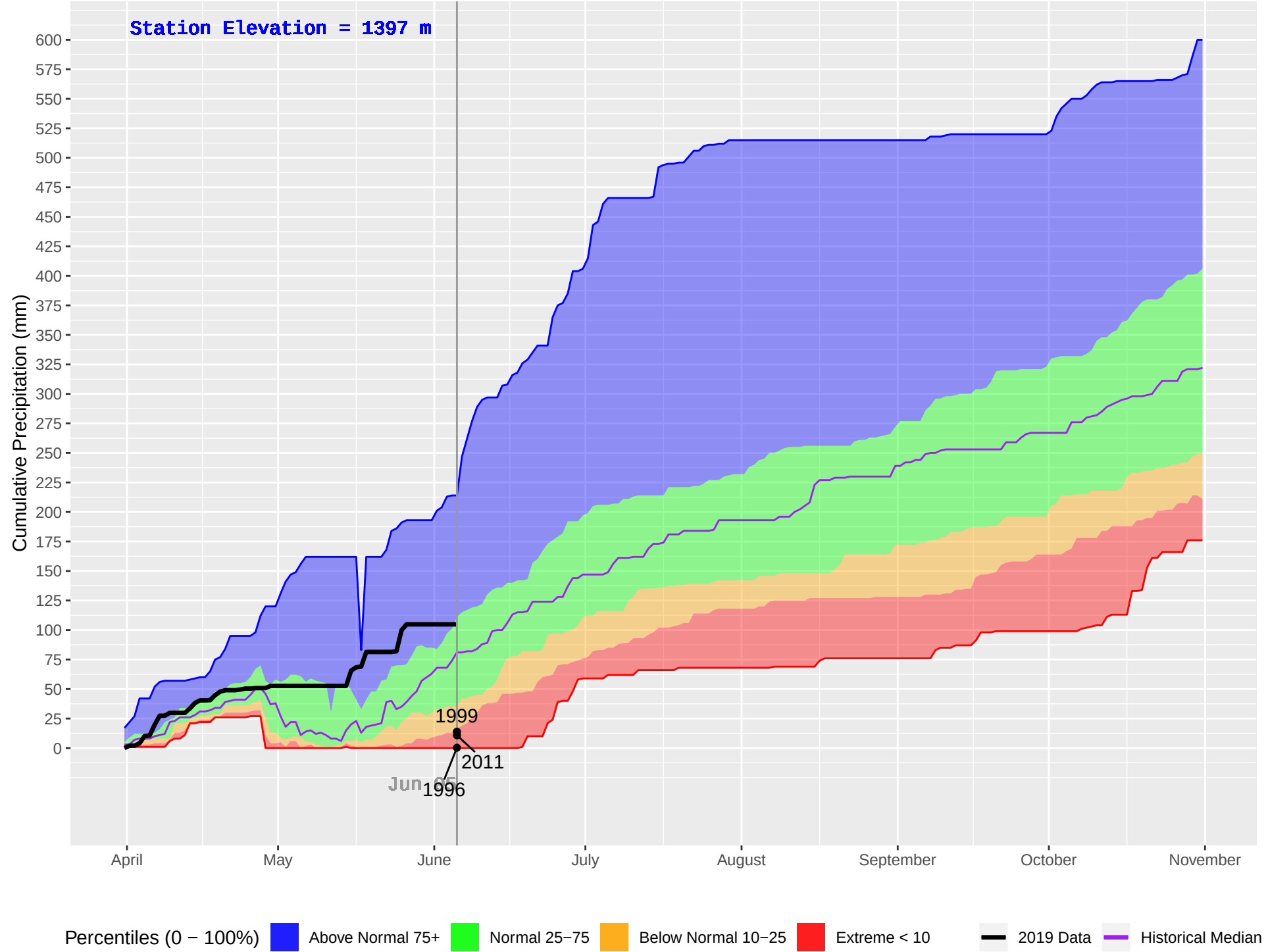
NANCY GREEN (407) : Historical (1992–2018), Current (2019) Daily Cumulative Precipitation
