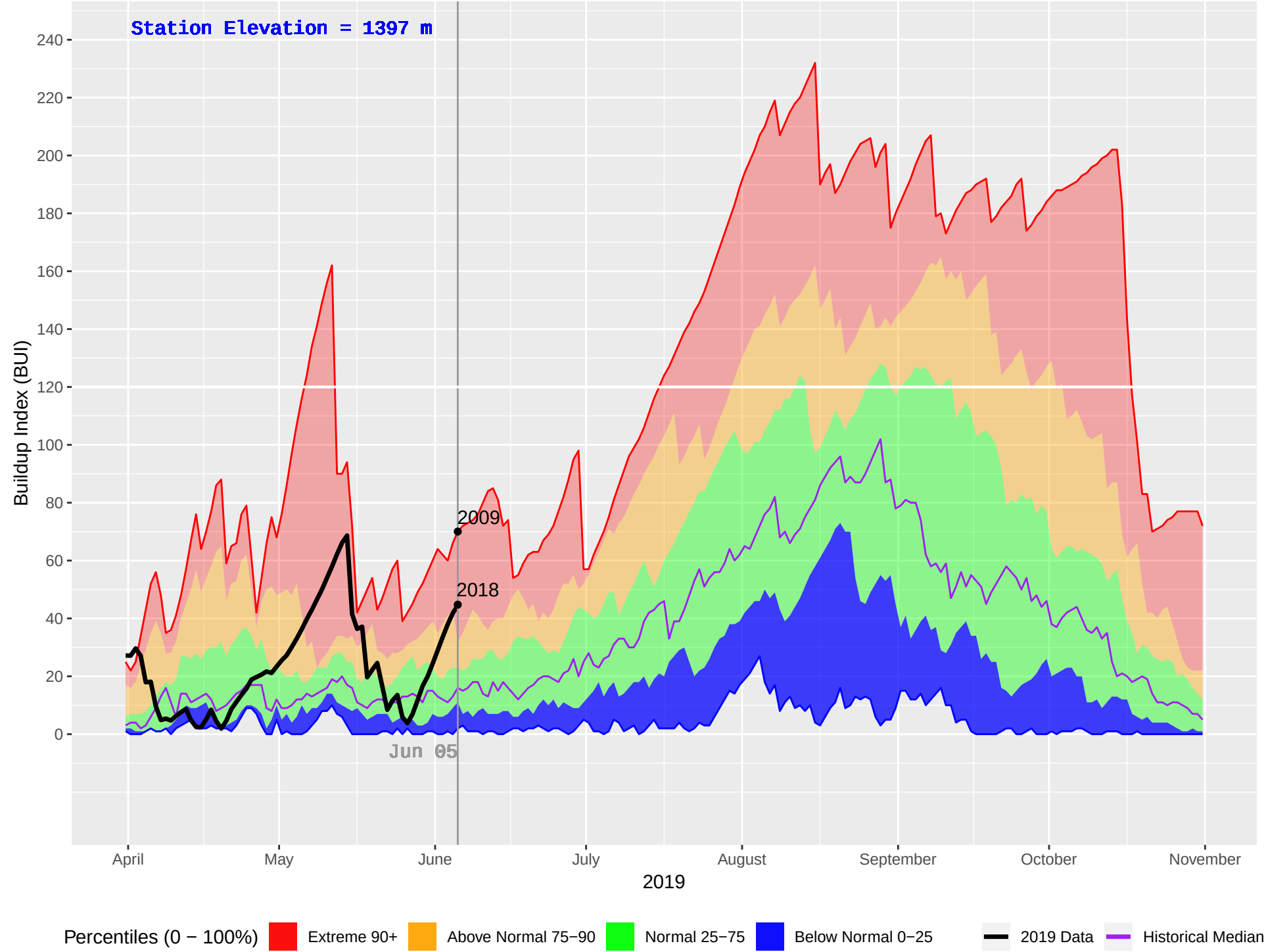
NANCY GREEN (407) : Historical (1992–2018), Current (2019) Daily Buildup Index (BUI)
